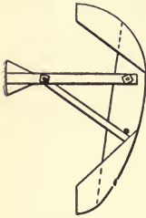
FIG. 9.—INSPECTOR'S TEMPLET FOR EGG- SHAPED SEWER.
